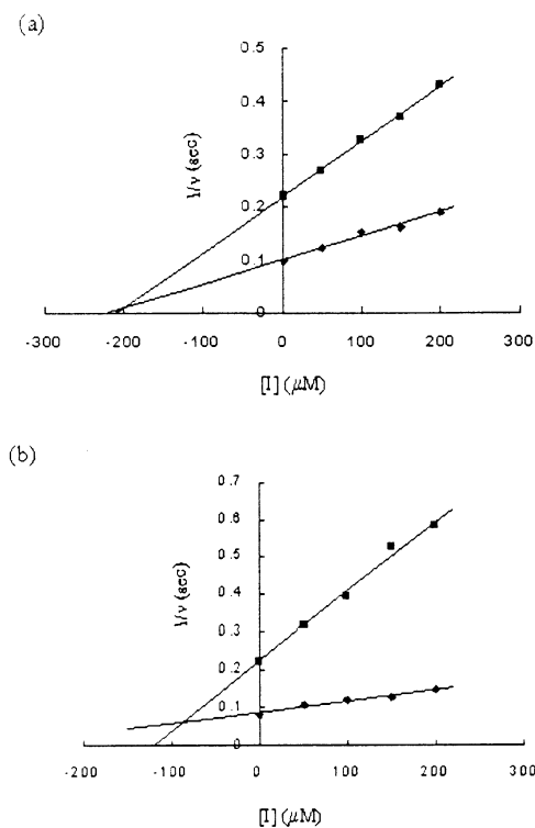
Figure 7. Dixon plots for determinations of K_S values in the acylation reactions of α-CT with (a) (R)- 1 and (b) (S)- 1 . Assay conditions are found in Experimental.
