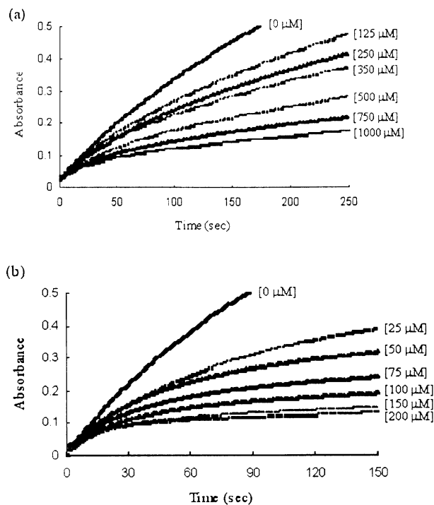
Figure 5. Progress curves showing the \alpha -CT catalyzed hydrolysis of Succ-AAPF-pNA in the presence of varied concentrations of (a) ( R )- 1 and (b) ( S )- 1 . Assay conditions are described in Experimental.
