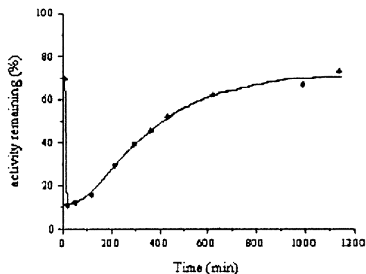
Figure 2. Spontaneous reactivation of \alpha -CT inactivated by 1 at 25 °C in 0.05 M Tris buffer pH 7.5 containing 20% DMSO. The final concentrations of \alpha -CT and 1 are 25 nM and 1.25 \mu\text{M} , respectively. The enzymic activity was assayed using Suc-AAPF- p NA (125 \mu\text{M} ) as the substrate.
