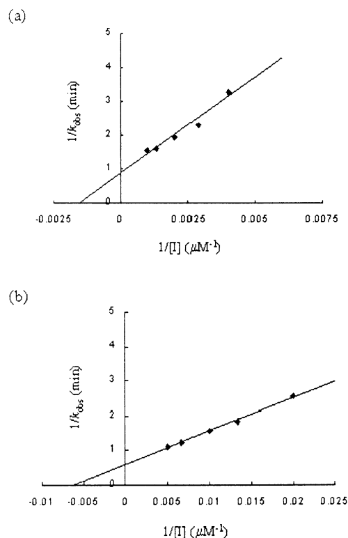
Figure 6. Kitz–Wilson plots for determinations of K_M and k_a values for (a) (R)- 1 and (b) (S)- 1 .
