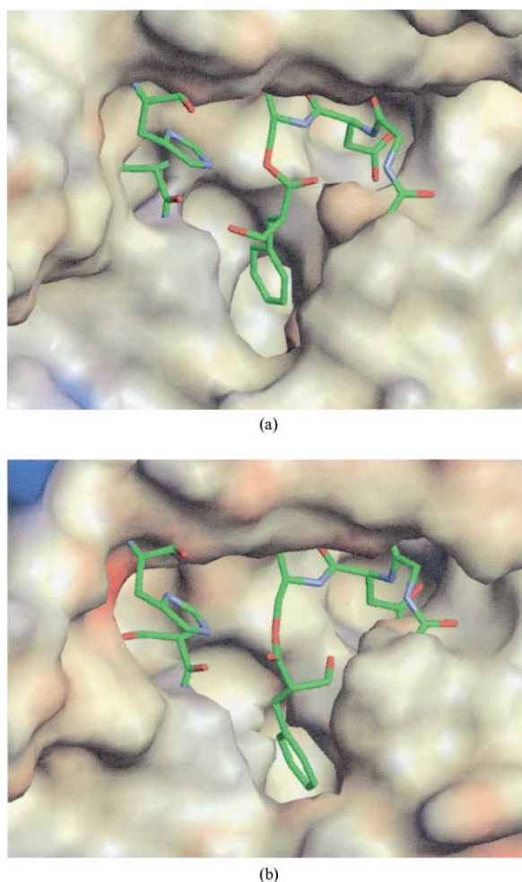
Figure 9. Computer generated models of the active site of \alpha -CT whose Ser-195 hydroxyl is acylated by (a) ( R )- 1 and (b) ( S )- 1 .
