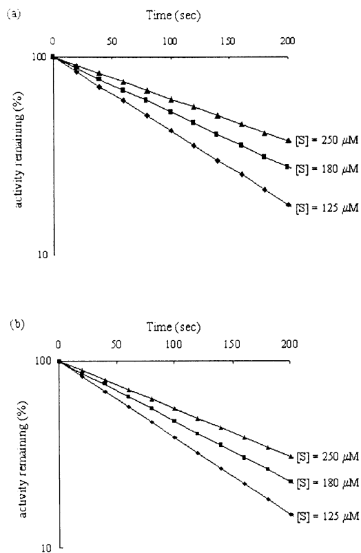
Figure 4. Active site protection tests for (a) ( R )- 1 ( [\alpha\text{-CT}] = 25 nM, [(R)\text{-1}] = 500 μM, and [\text{Succ-AAPF-pNA}] = 125, 180, and 250 μM), and (b) ( S )- 1 ( [\alpha\text{-CT}] = 25 nM, [(S)\text{-1}] = 200 μM, and [\text{Succ-AAPF-pNA}] = 125, 180, and 250 μM).
