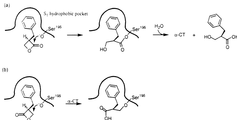
Figure 1. Postulated reaction paths of (a) ( R )- 1 and (b) ( S )- 1 at the active site of \alpha -CT.
