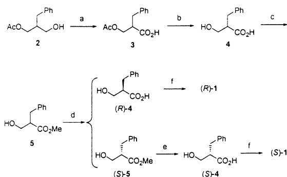
Scheme 1. Reagents, conditions, and (yields): (a) Jones' reagent, 0 °C (73%); (b) \text{K}_2\text{CO}_3 , MeOH/ \text{H}_2\text{O} (90%); (c) \text{H}^+ , MeOH (86%); (d) \alpha -CT, 0.05 M phosphate buffer (pH 7.5); (e) (i) \alpha -CT, 0.05 M phosphate buffer (pH 7.5); (ii) LiOH, MeOH/ \text{H}_2\text{O} (70%); (f) \text{Ph}_3\text{P} , DMAD, -78 °C (75%).
