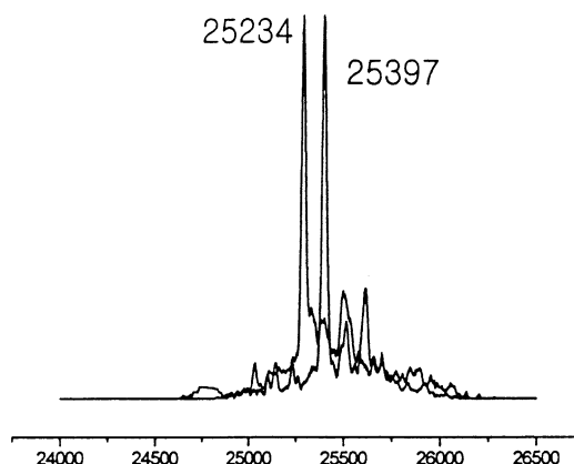
Figure 3. Superimposed electrospray mass spectra of \alpha -CT ( m/z 25234 Da) and \alpha -CT complexed with ( R )- 1 ( m/z 25397 Da).
