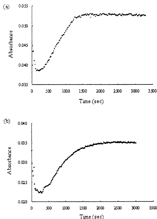
Figure 8. The determinations of k_d values for (a) ( R )- 1 and (b) ( S )- 1 by the proflavin displacement assay method.
